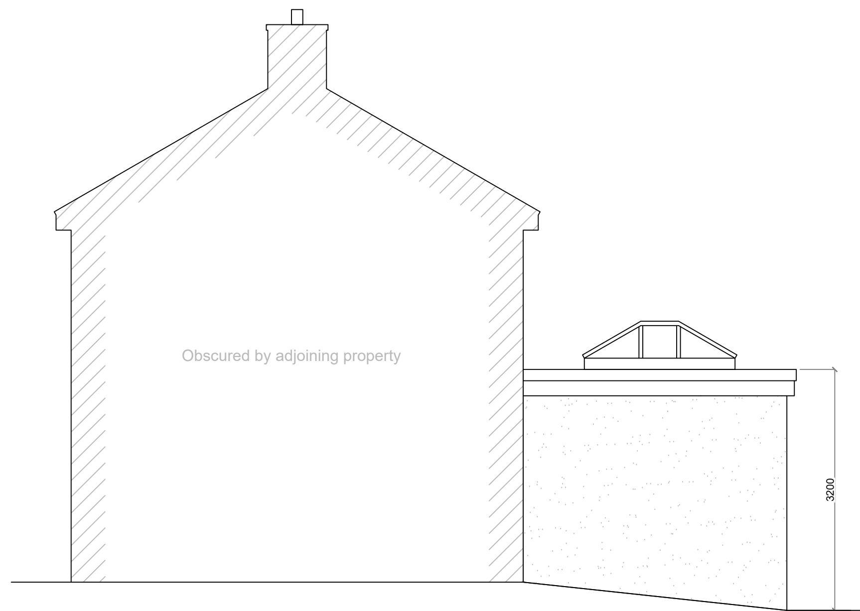
West Elevation
