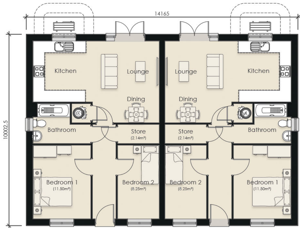
TYPE B 2B3P 61 Bungalow (AS) GROUND FLOOR PLAN - Semi-Detached TYPE B 2B3P 61 Bungalow (OPP)
