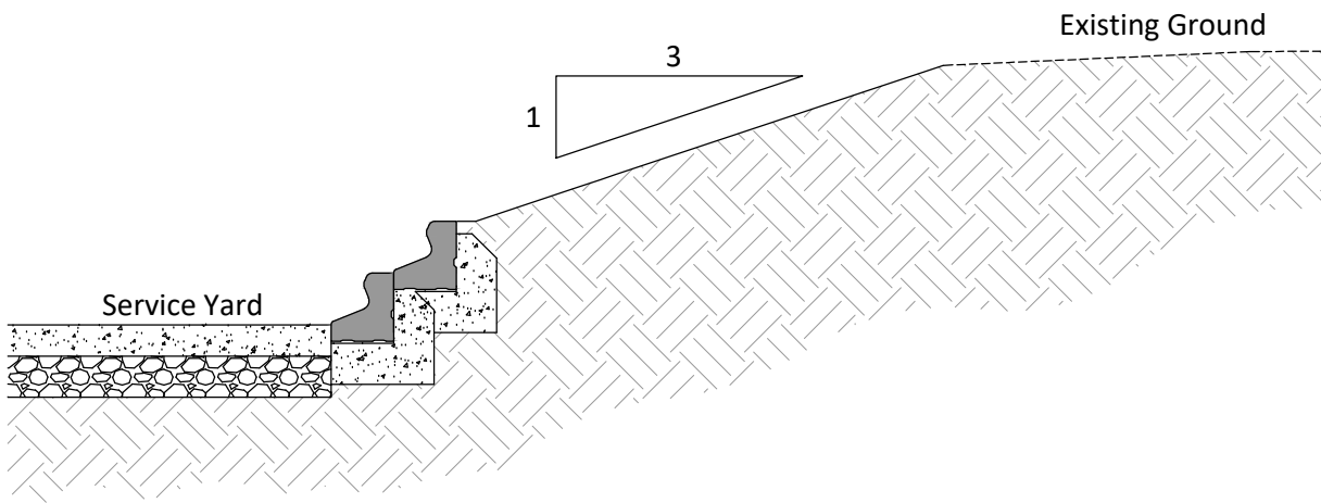
Section through Double Trief Scale 1:50
