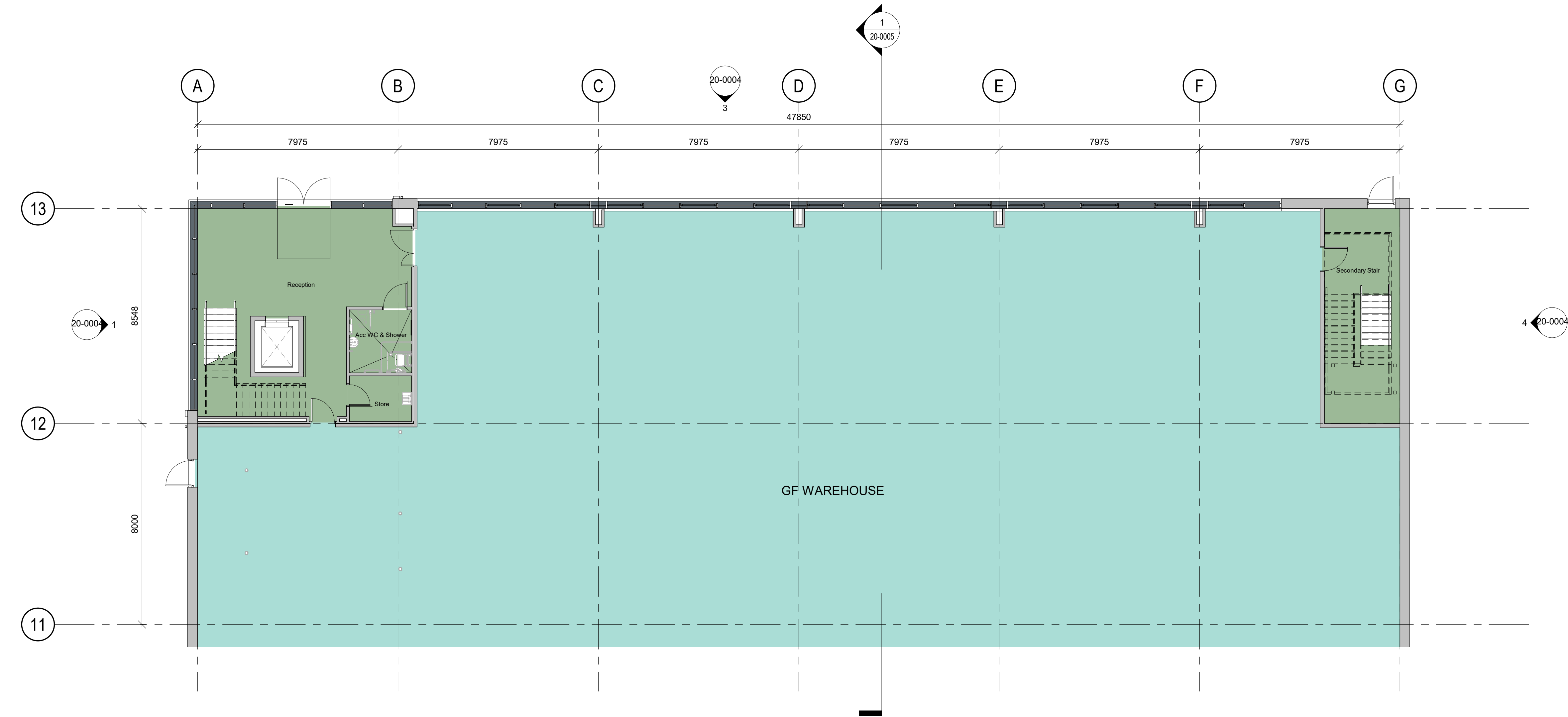
Ground Floor Office GA Plan 1:100
