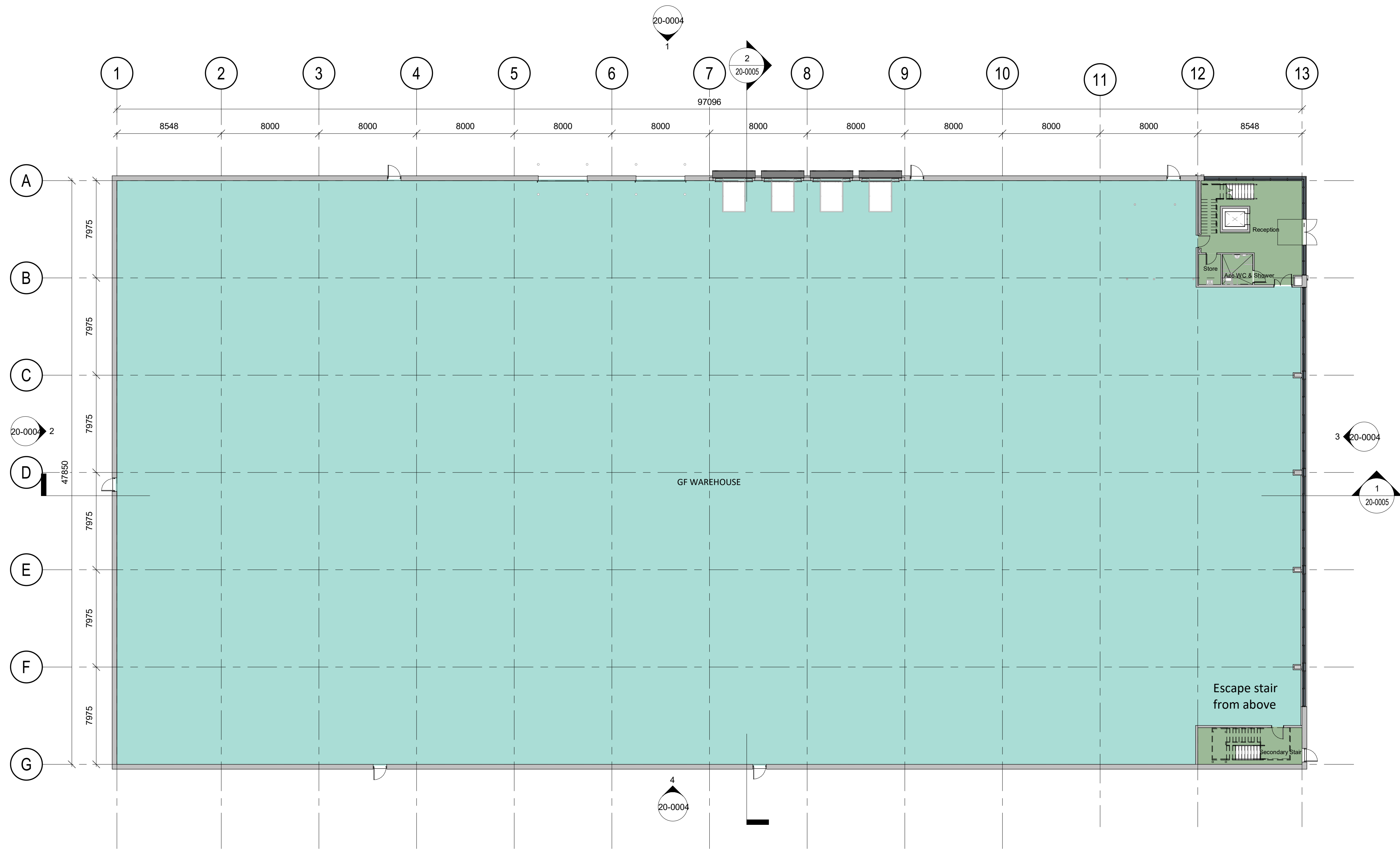
Ground Floor GA Plan 1:200
