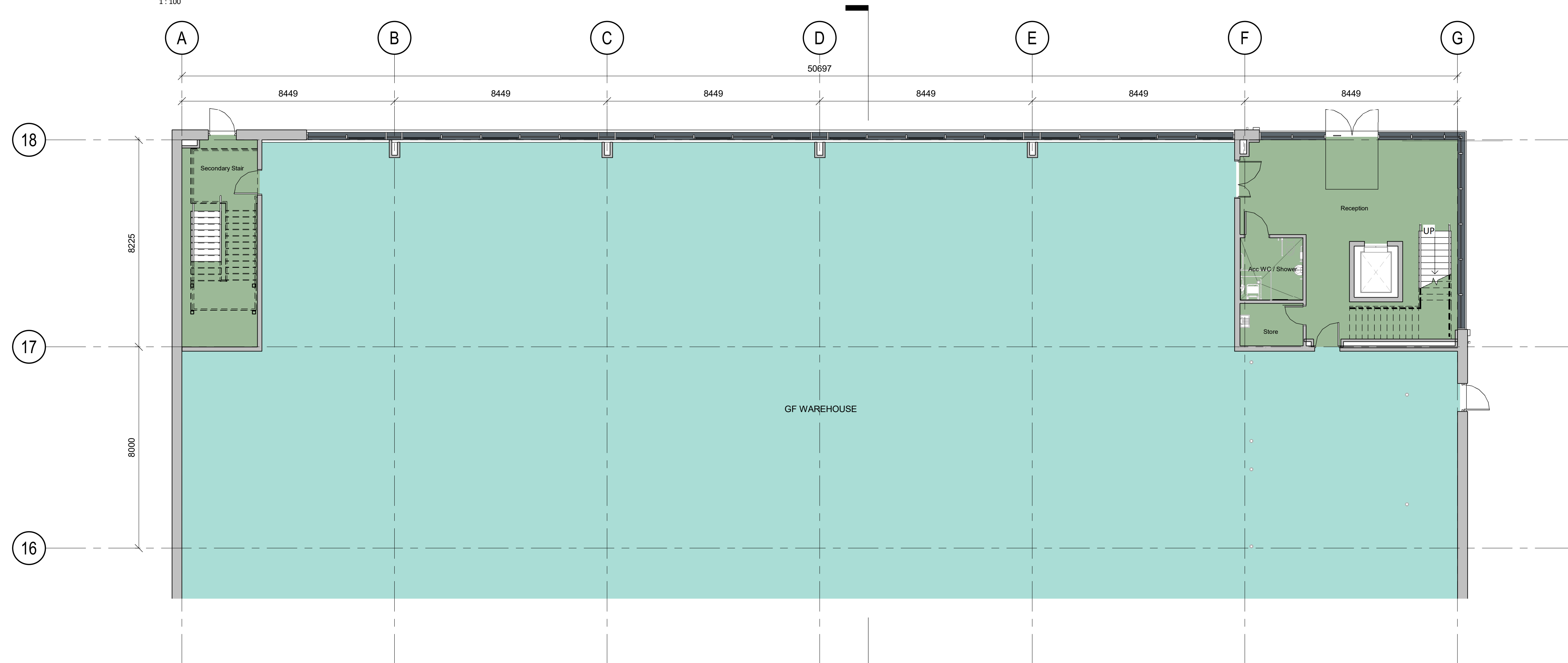
Ground Floor Office GA Plan 1 : 100
