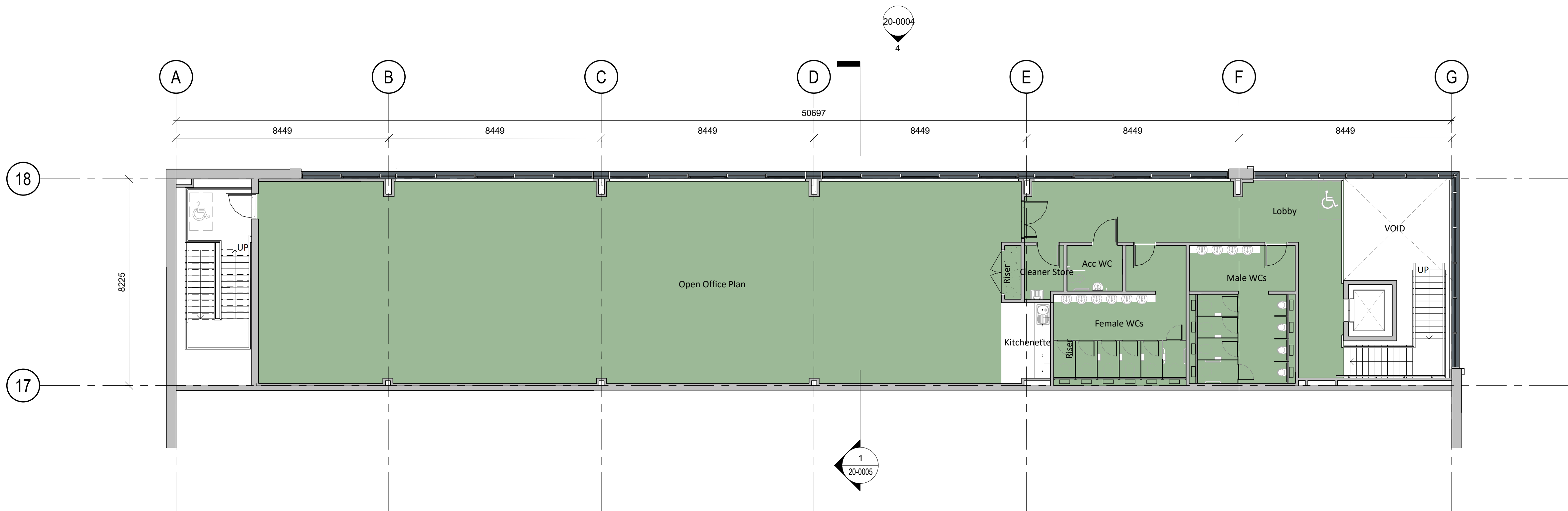
First Floor Office GA Plan 1 : 100
