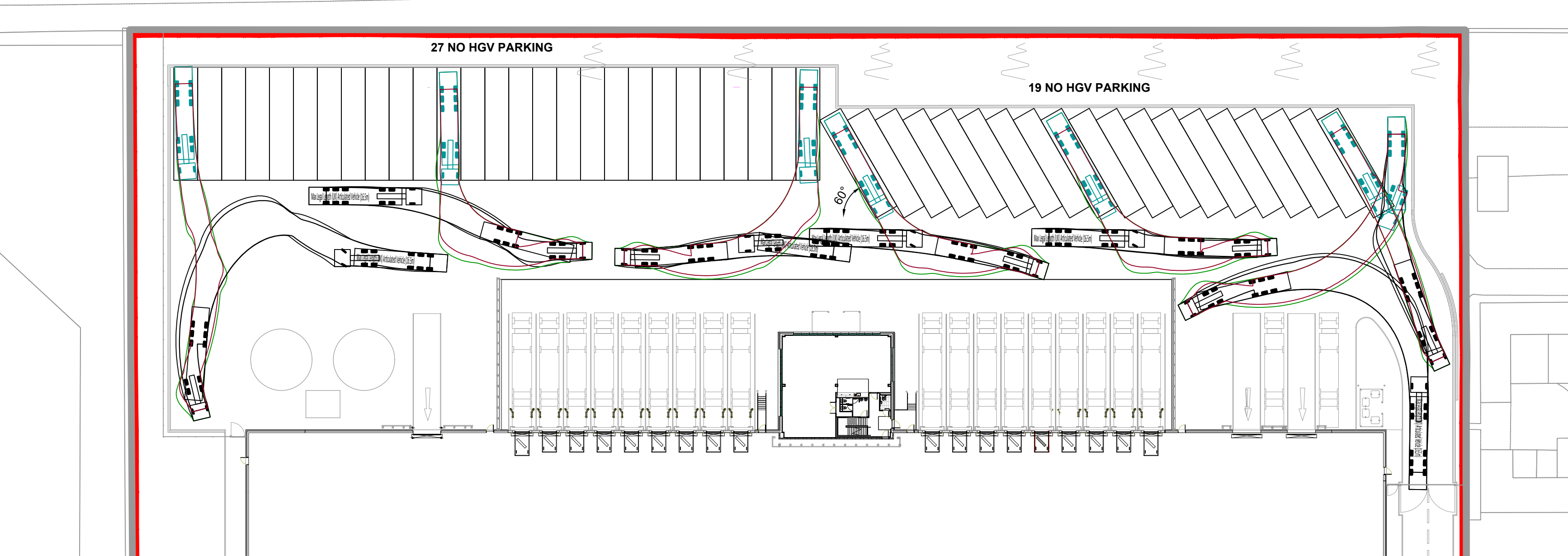
Vehicle Tracking - HGV Reverse Parking Scale 1:500
