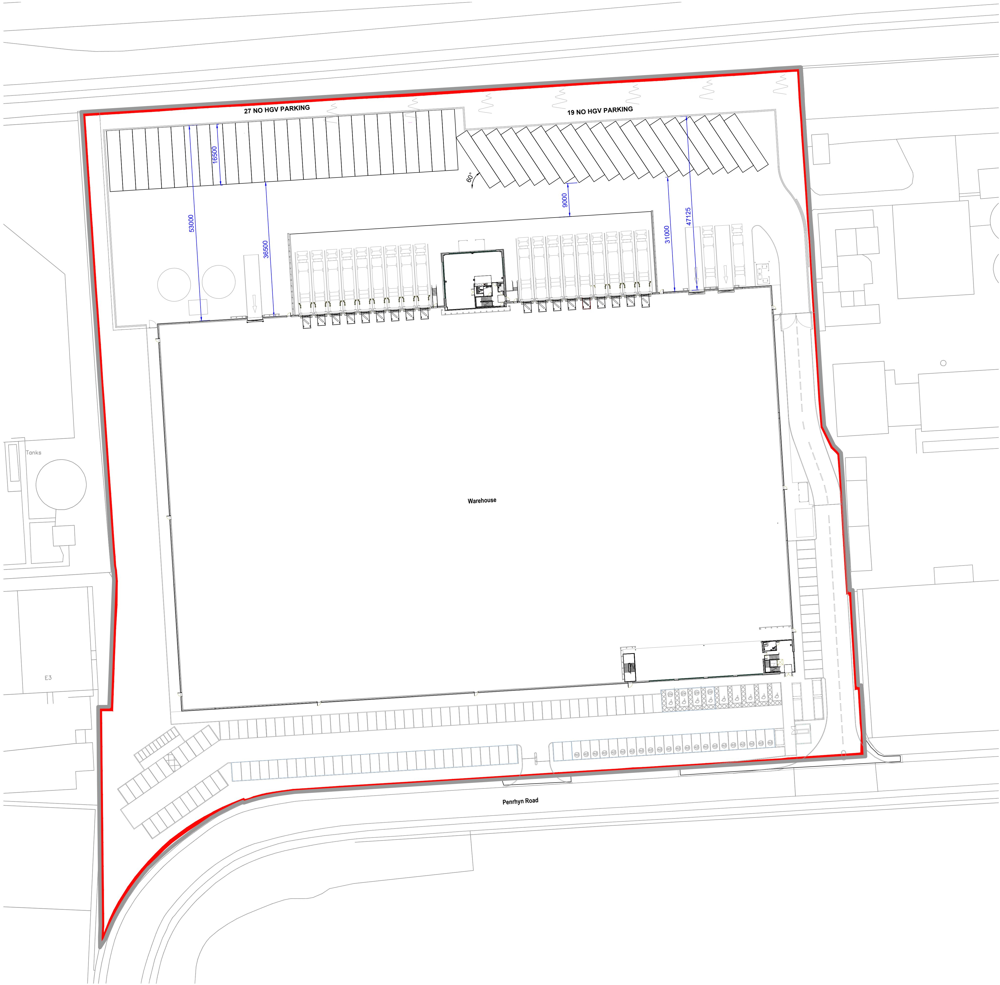
Proposed Site Layout Scale 1:500
