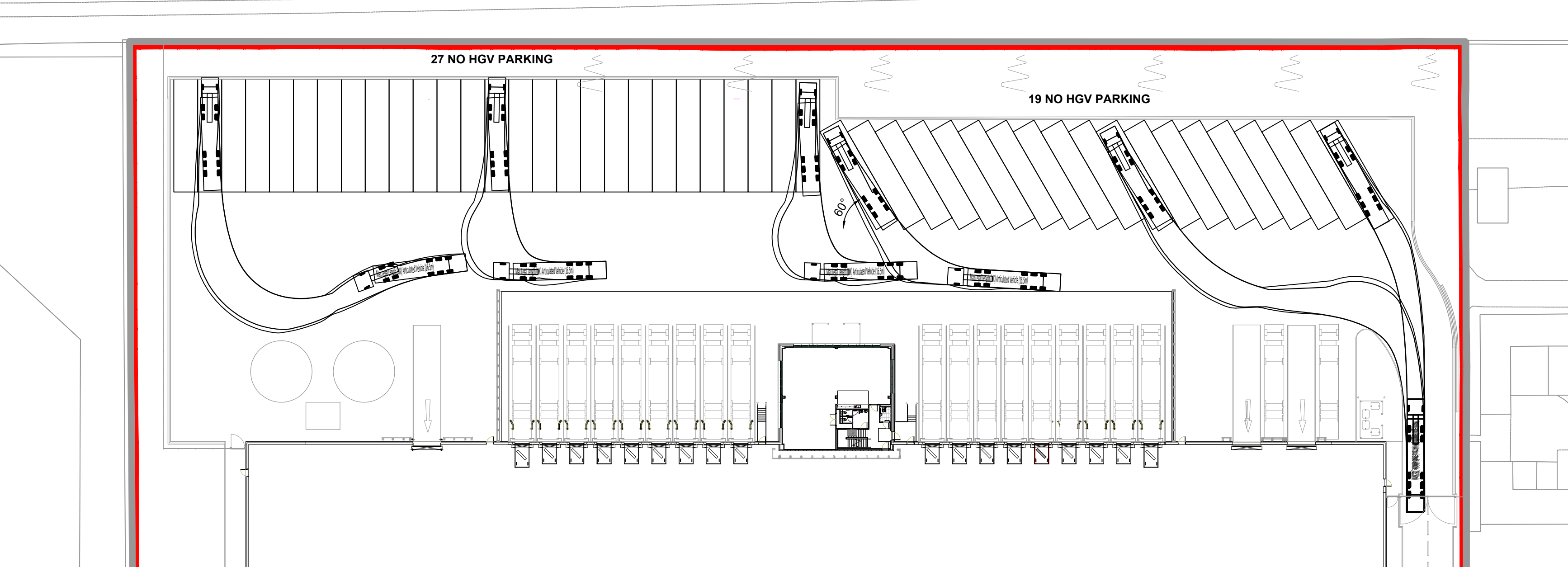
Vehicle Tracking - HGV Forward Parking Scale 1:500
