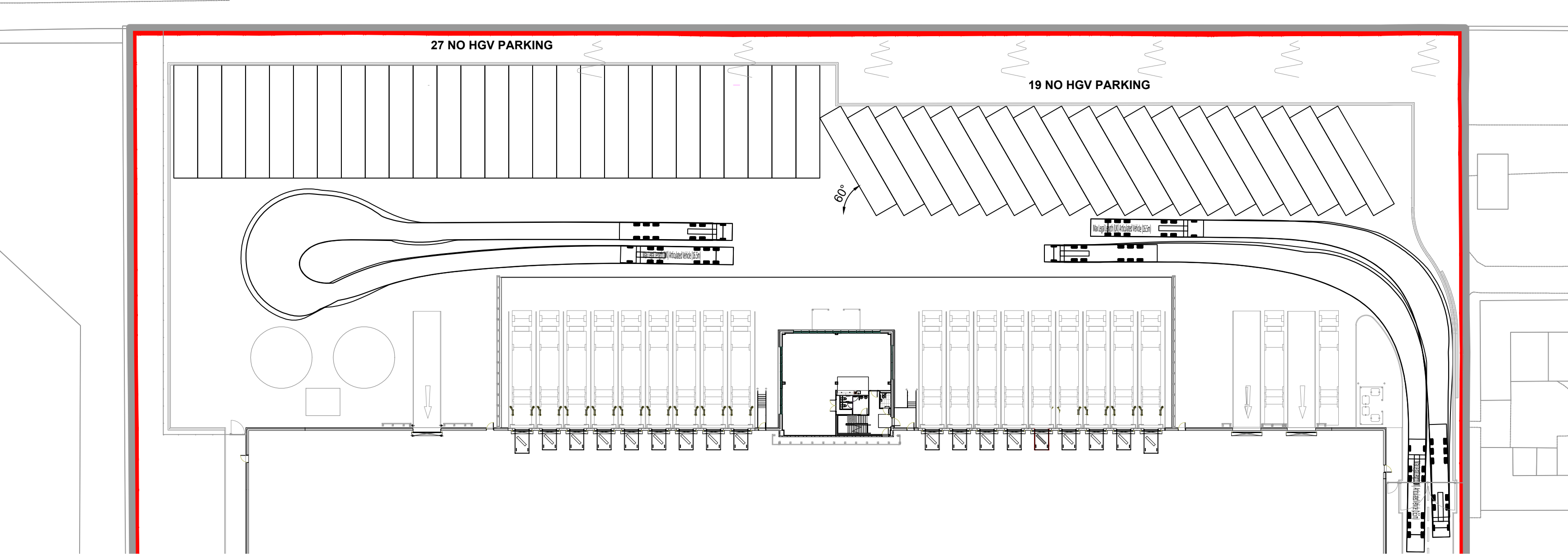
Vehicle Tracking - Site Maneuvering Scale 1:500
