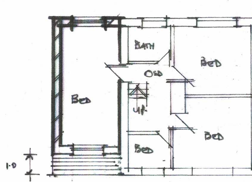
Prop First Floor Plan
