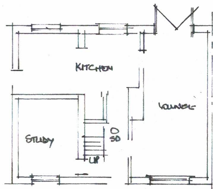
Prop Ground Floor Plan
