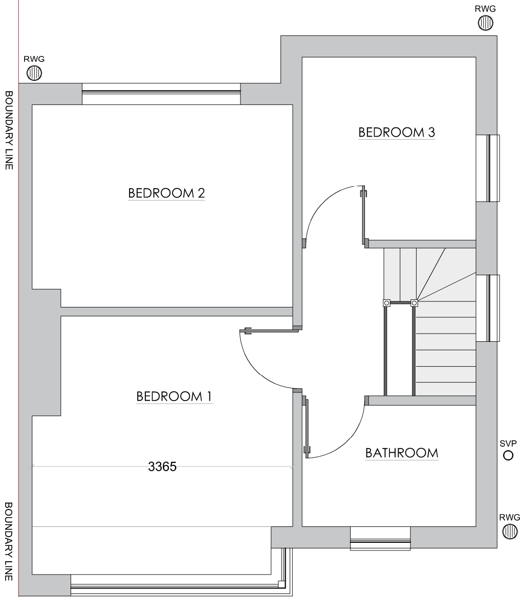
EXISTING FIRST FLOOR (Scale 1:50)
