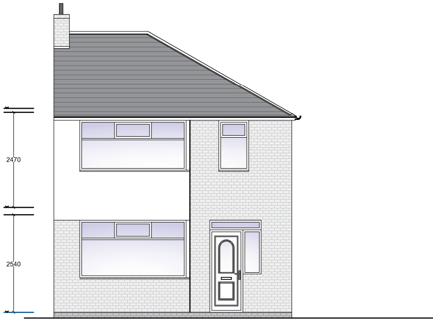
EXISTING FRONT ELEVATION (Scale 1:100) SCALE BAR - (mm) 500 1000 2000
