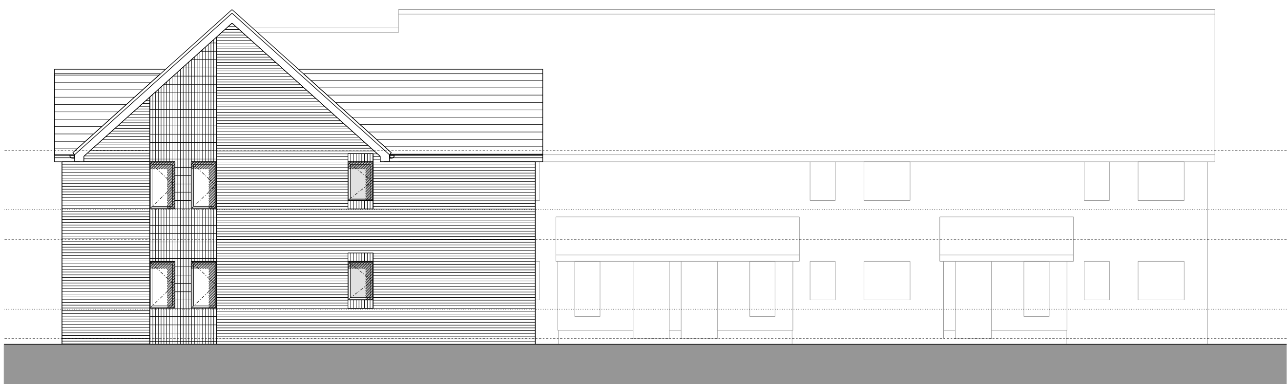
FRONT ELEVATION
