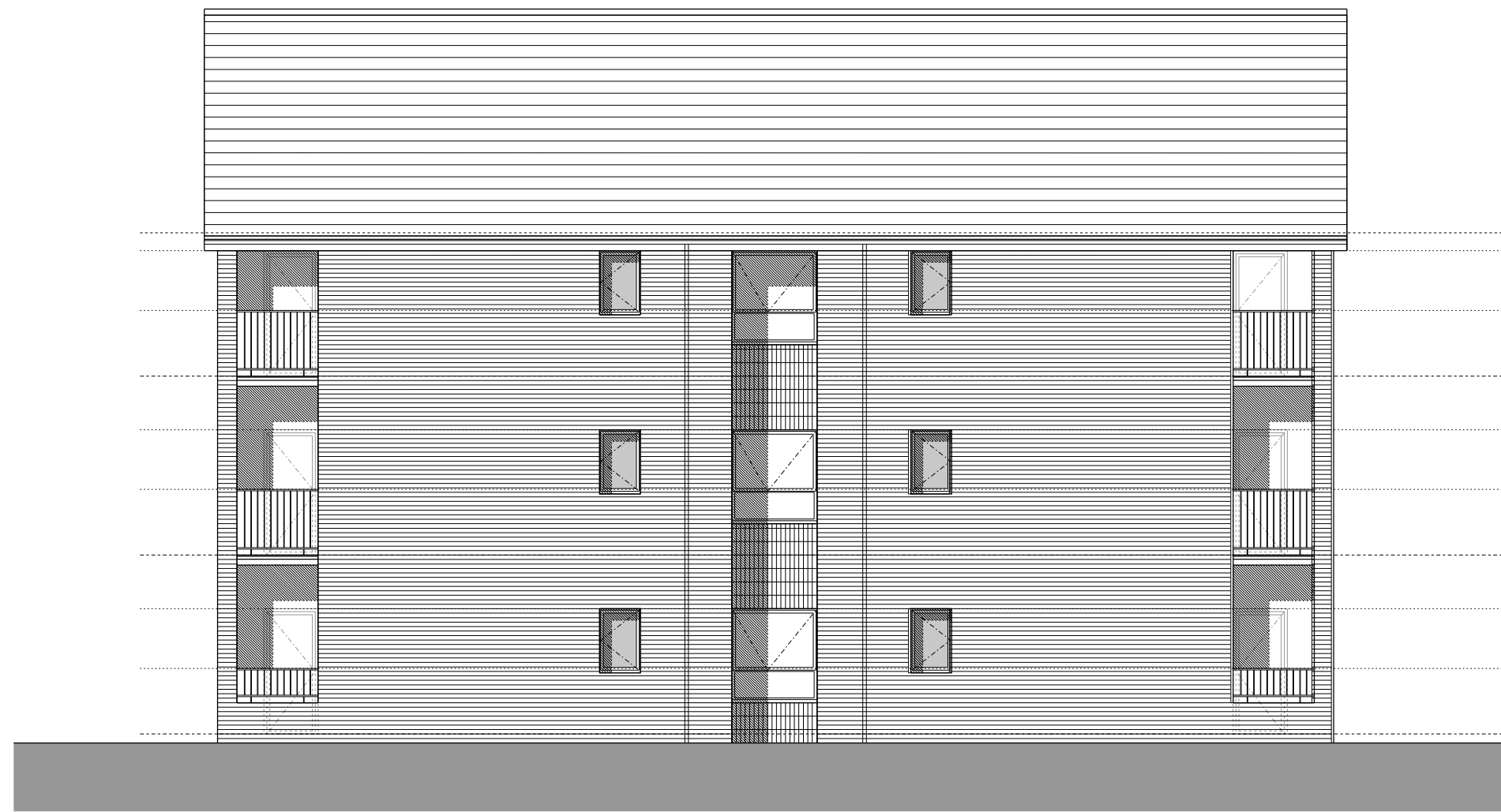
SIDE ELEVATION
