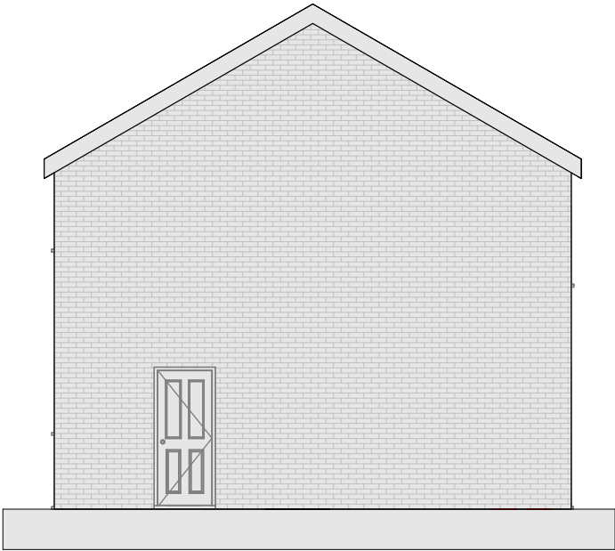
Existing West 1 : 100
