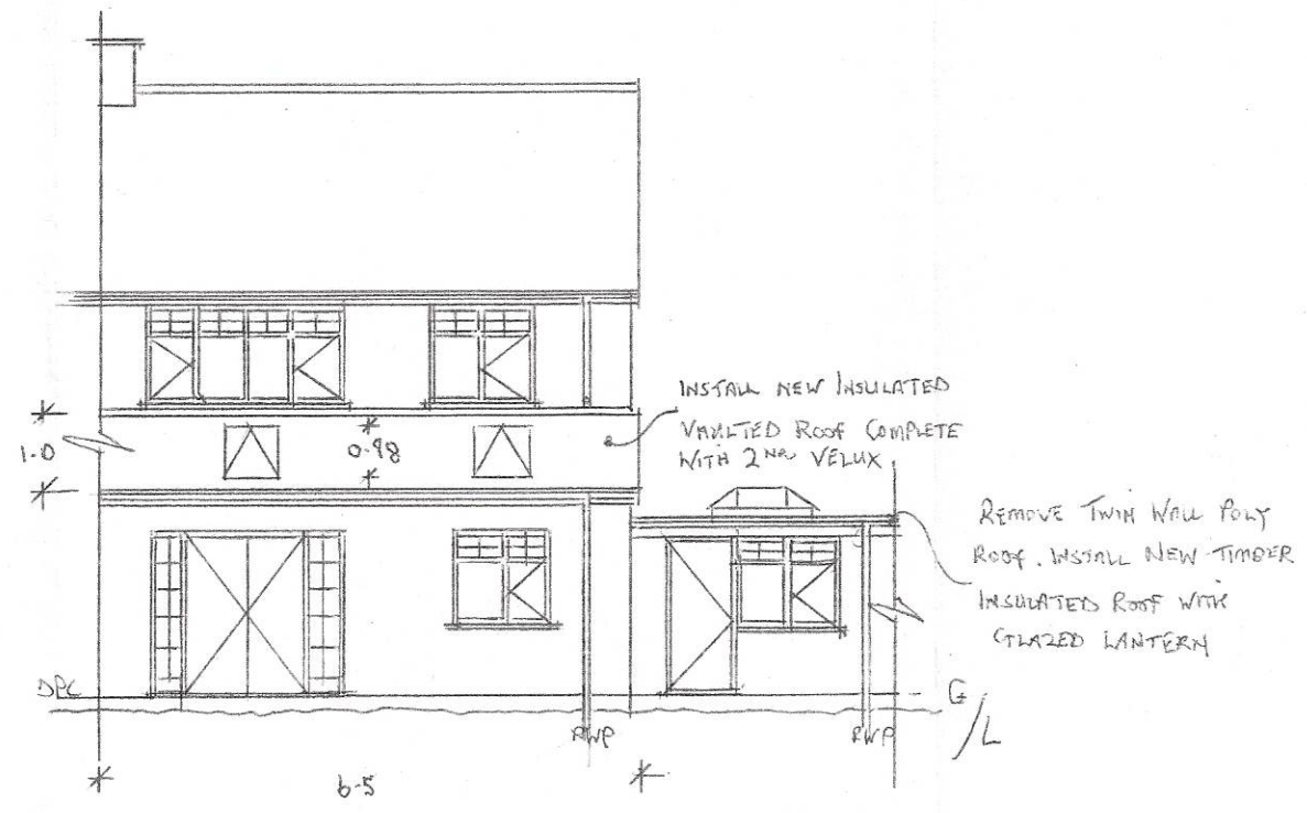
PROPOSED REAR
