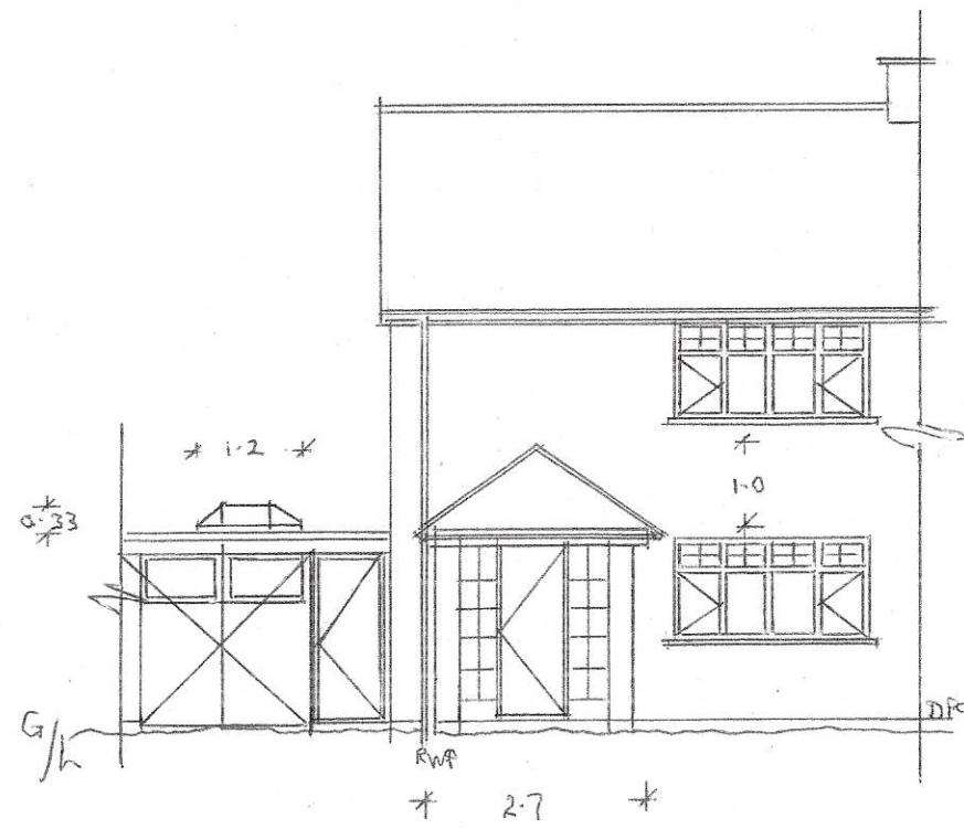
PROPOSED FRONT
