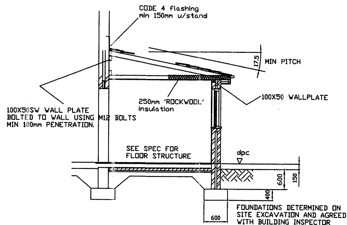
TYPICAL SECTION THRO SINGLE STOREY STRUCTURE SCALE NTS
