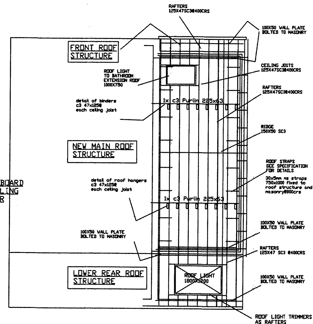
PLAN ON ROOF STRUCTURES SCALE 1:100
