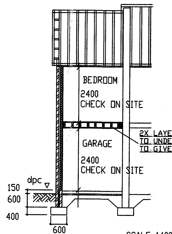
TYPICAL SECTION THRO ON EXTENSION
