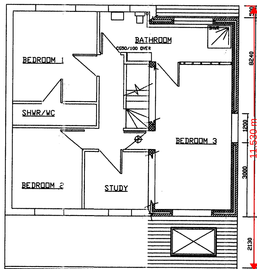
PLAN ON PROPOSED FIRST FLOOR WITH FLOOR STRUCTURE REMOVED
