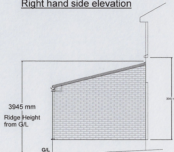
Right hand side elevation
