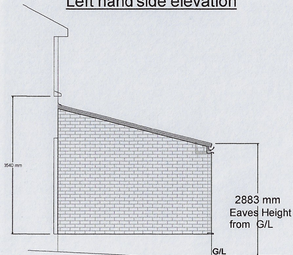
Left hand side elevation
