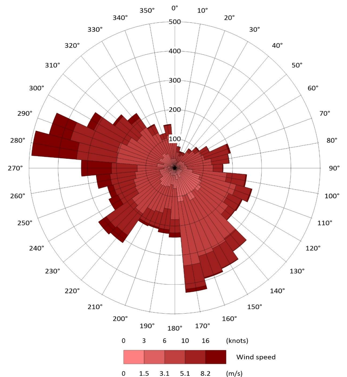
Figure 3: Wind Rose of 2019 Liverpool Airport Meteorological Data
