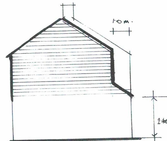
Prop Side Elevation
