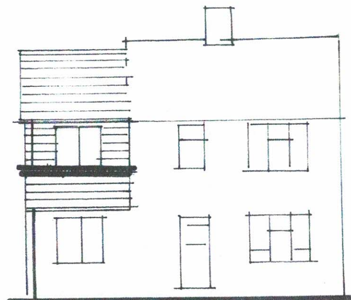
Prop Front Elevation
