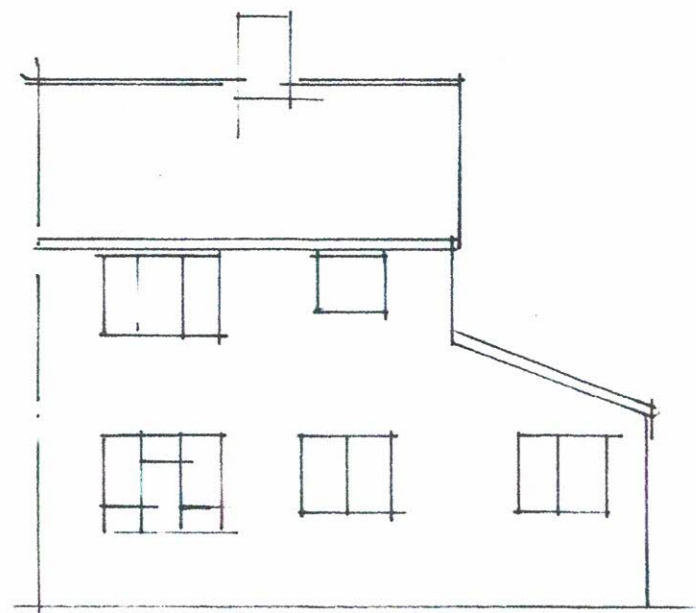
EXTG REAR ELEVATION 1:100
