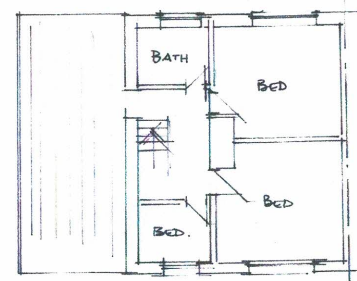
EXTG FIRST FLOOR PLAN 1:100
