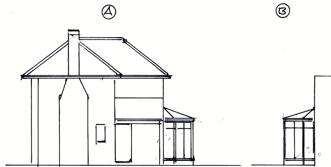
SIDE ELEVATIONS 1:100
