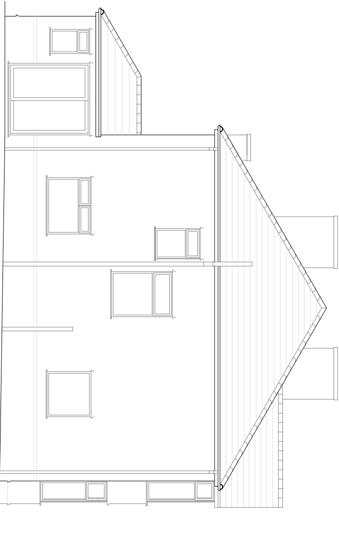
GABLE ELEVATION (EXISTING)
