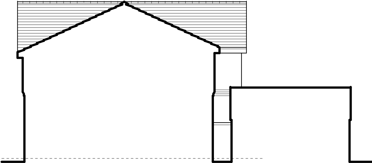
EXISTING RIGHT SIDE ELEVATION 1:100
