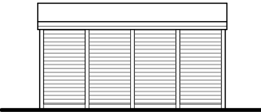
EXISTING SIDE ELEVATIONS 1:100
