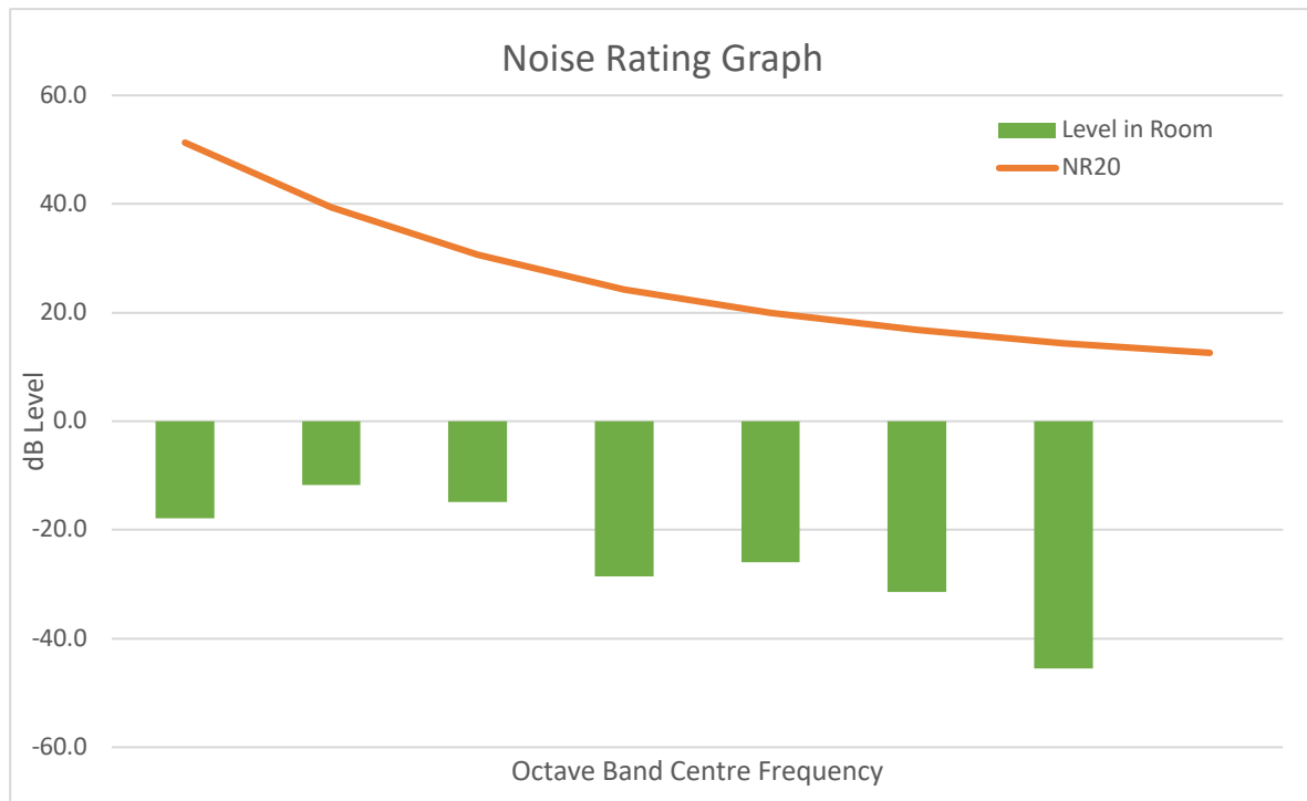
Figure 2: Predicted NR curve against NR20
