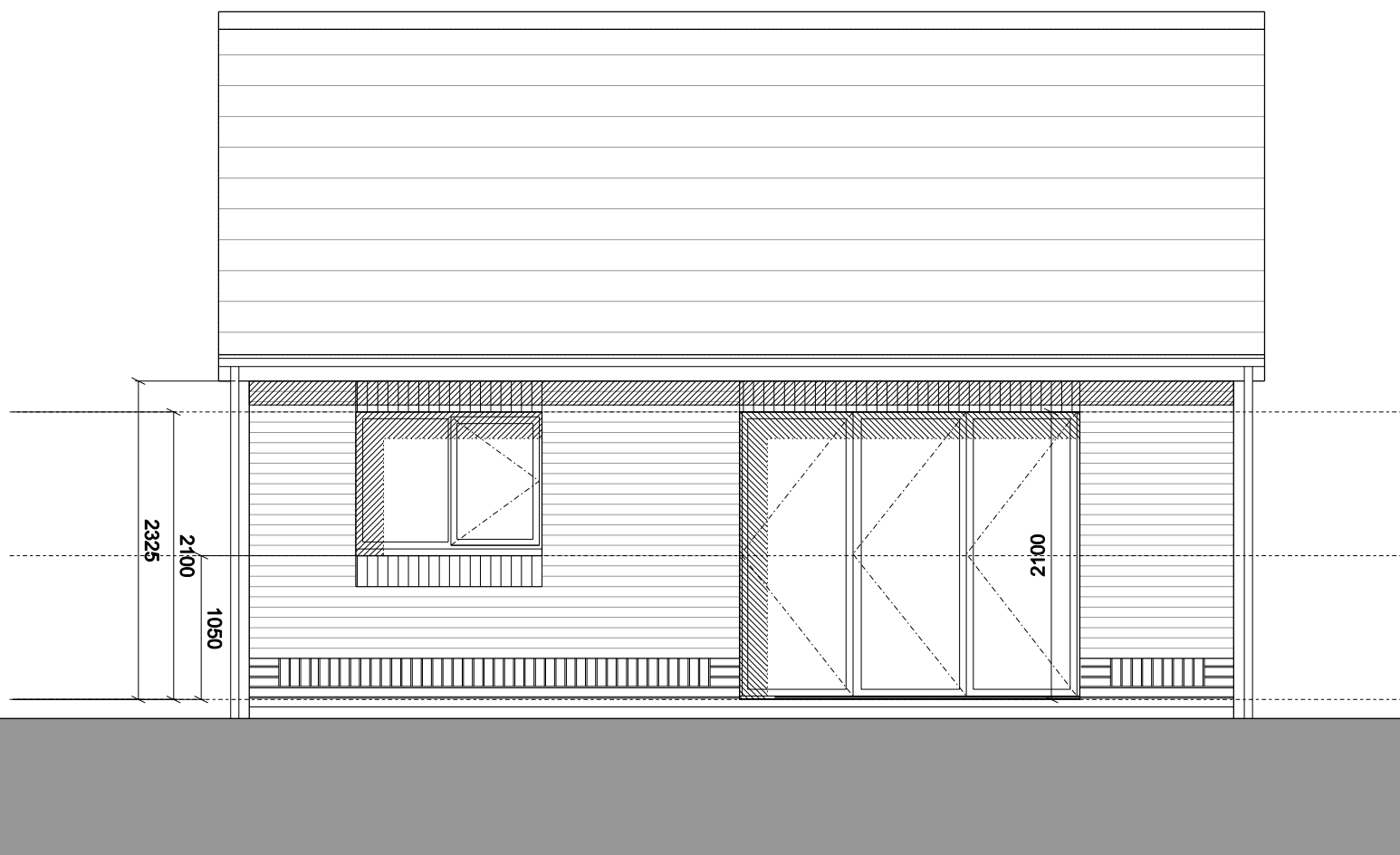
REAR ELEVATION
