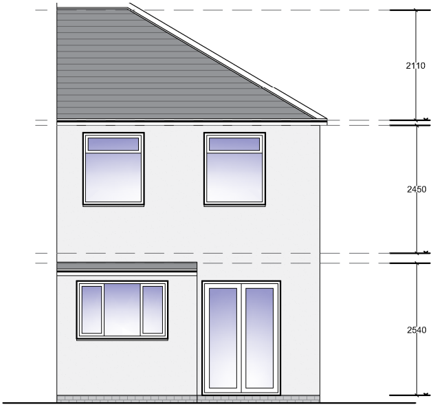
EXISTING REAR ELEVATION (Scale 1:100) 0 2000 1000 500 SCALE BAR - (mm)
