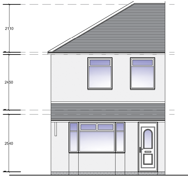
EXISTING FRONT ELEVATION (Scale 1:100) SCALE BAR - (mm) 0 500 1000 2000
