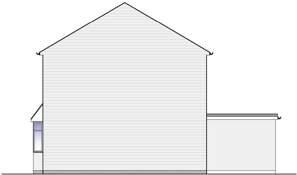
EXISTING SIDE ELEVATION (Scale 1:100) SCALE BAR - (mm) 0 500 1000 2000
