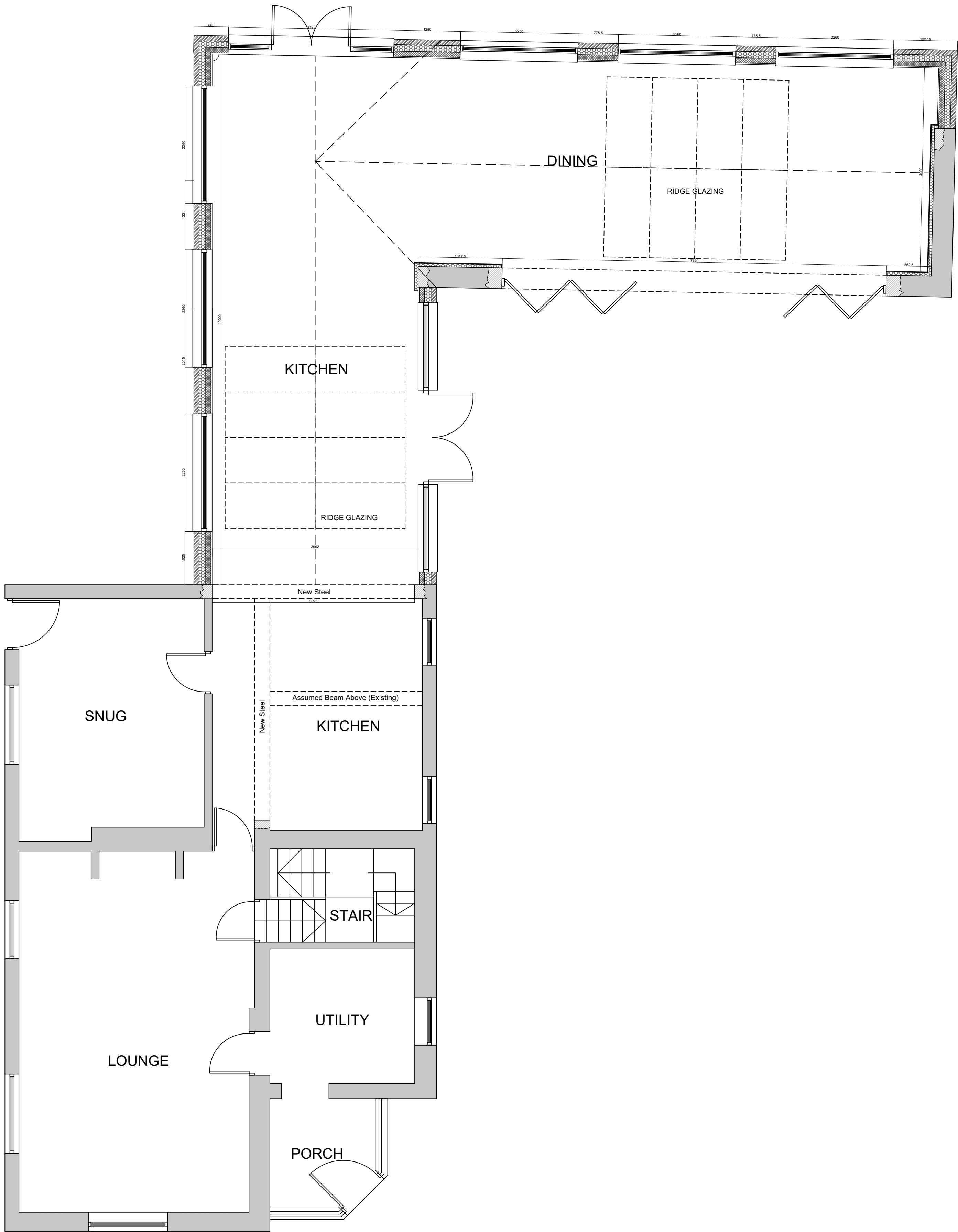
PROPOSED GROUND FLOOR 1:50
