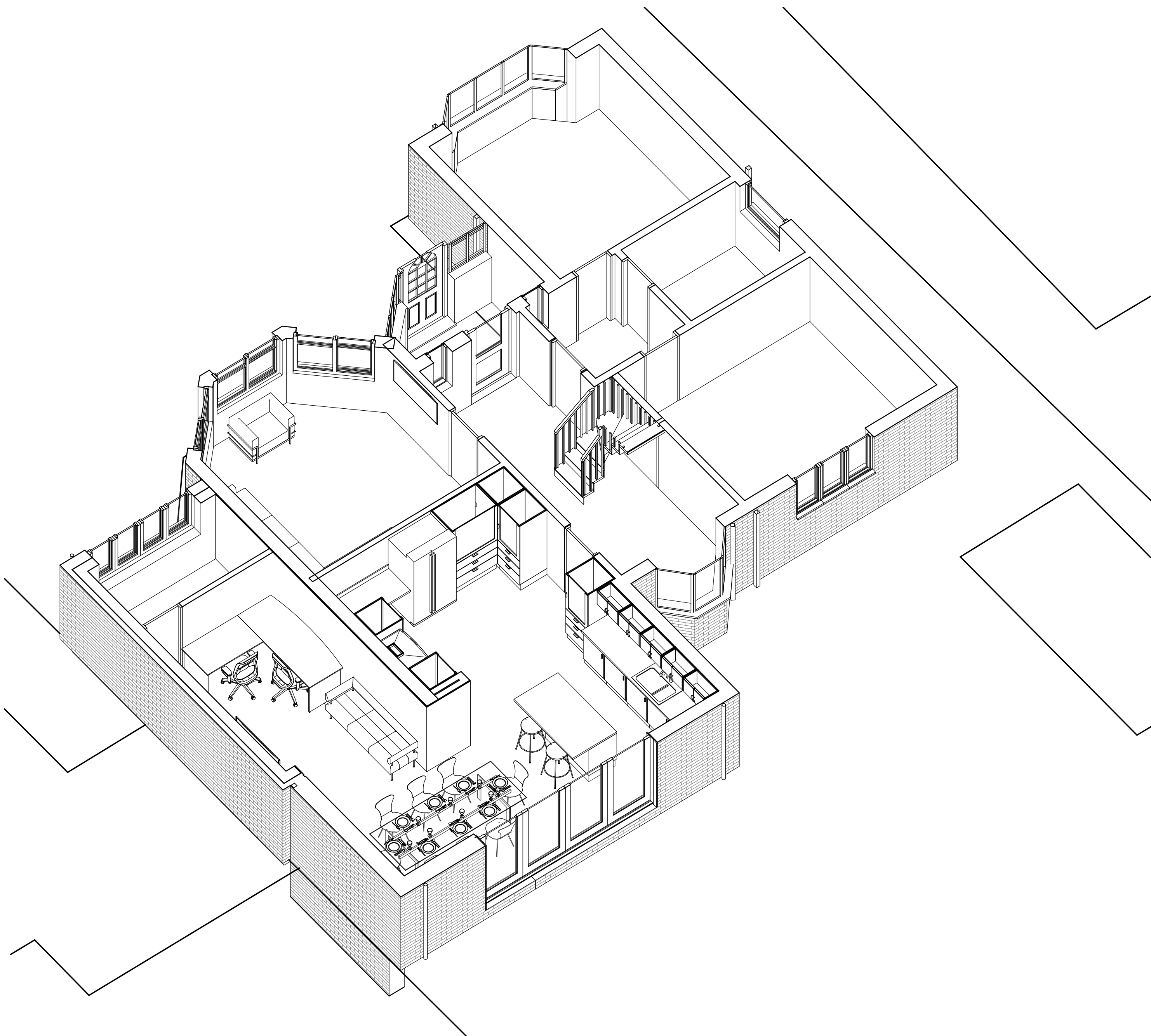
PROPOSED GROUND FLOOR 3D VIEW
