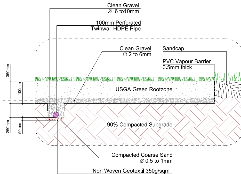
Typical Green Drainage GD01
