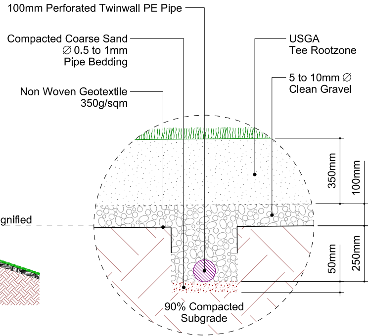
Typical Tee Drainage
