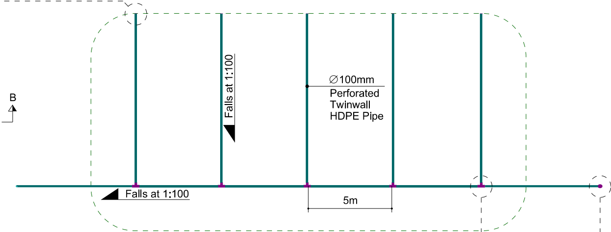
Typical Tee Drainage
