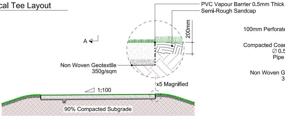
Section AA
