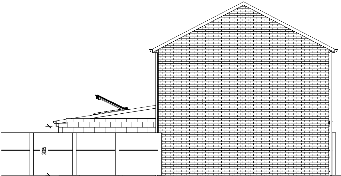
2 Blank Elevation Proposed 1 : 100
