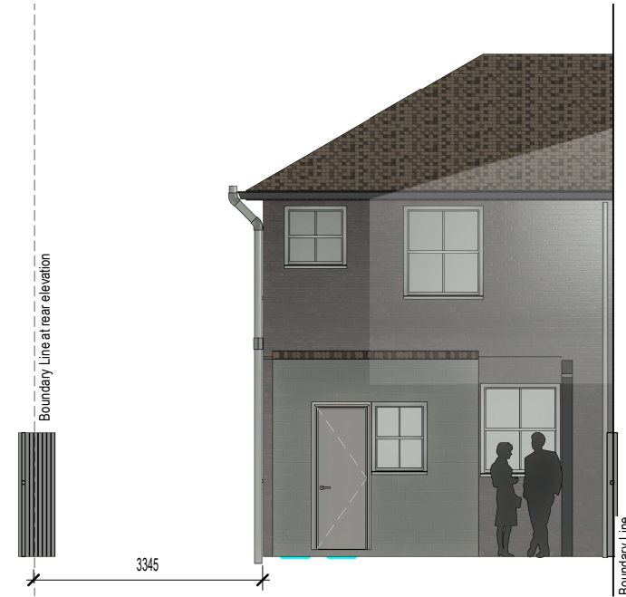
3 Existing Rear Elevation 1 : 100
