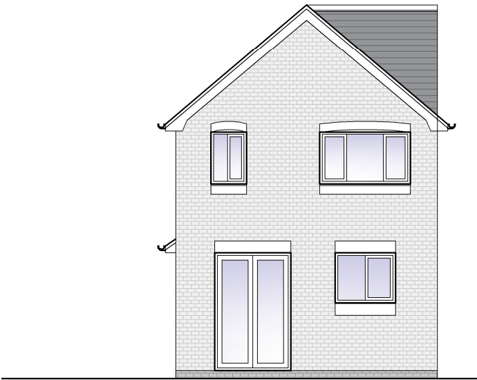
EXISTING REAR ELEVATION (Scale 1:100) 2000 1000 500 SCALE BAR - (mm)
