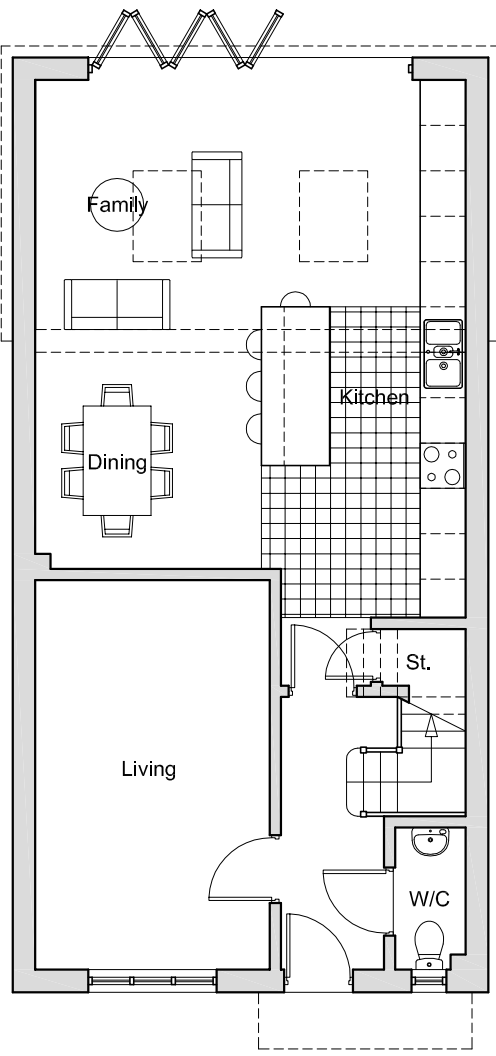
Proposed G/F Plan 1:100
