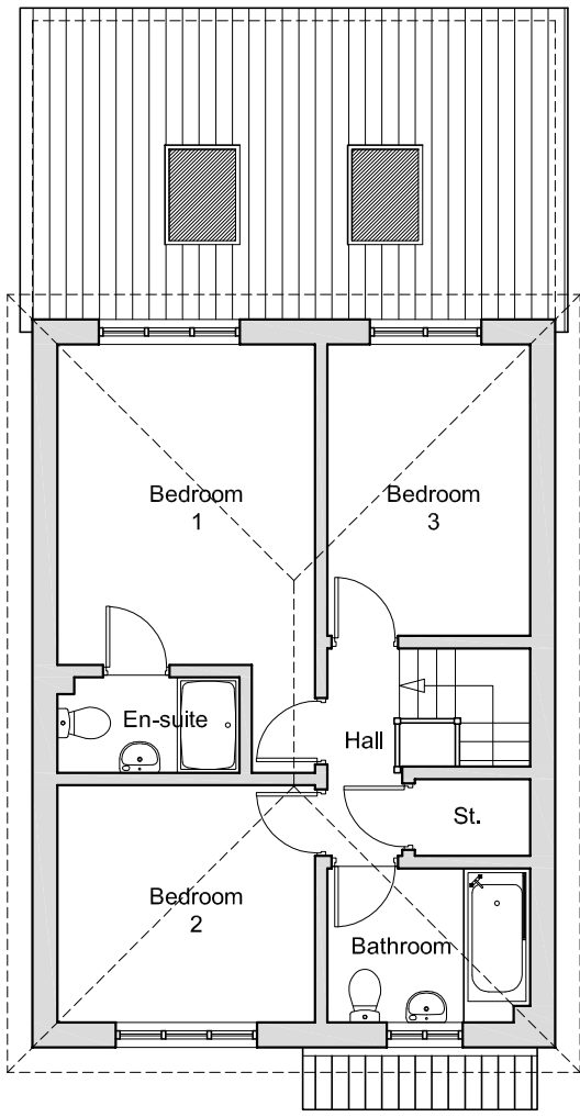
Proposed 1/F Plan 1:100
