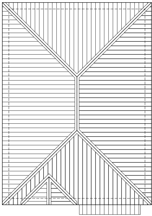
Existing Roof Plan 1:100
