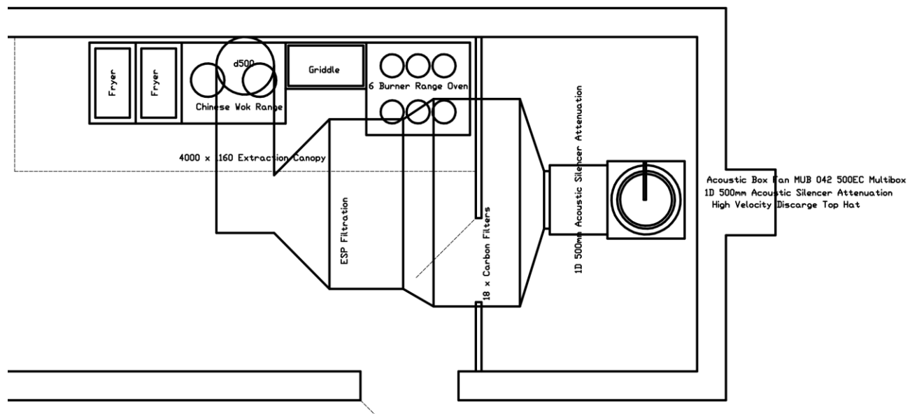
Figure 1: Top-Down View of Ventilation System
