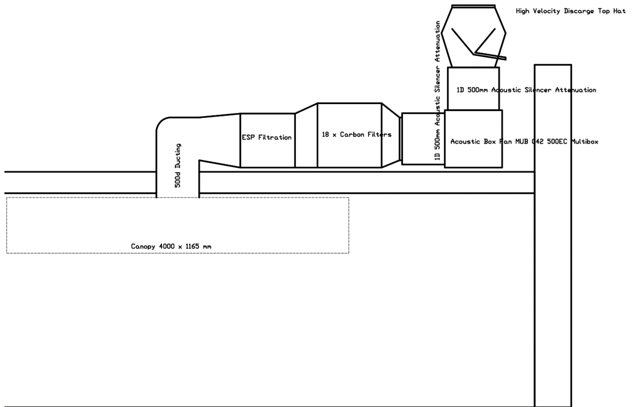
Figure 2: Side View of Ventilation System
