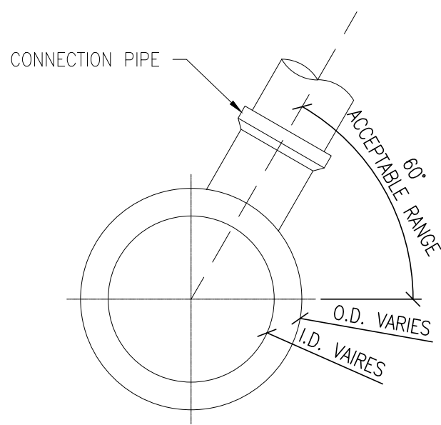
CROSS-SECTION VIEW OF SADDLE CONNECTION SCALE 1:10
