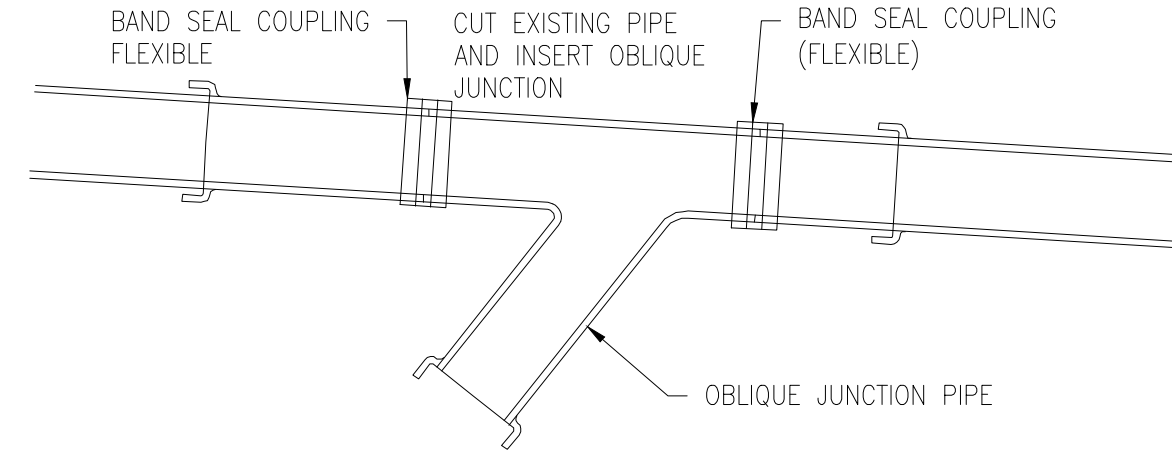
OBLIQUE JUNCTION / BAND SEAL COUPLING SCALE 1:25
