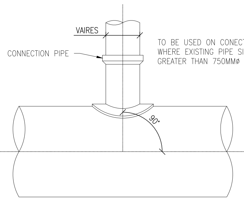
SIDE VIEW OF 90° SADDLE CONNECTION SCALE 1:10
