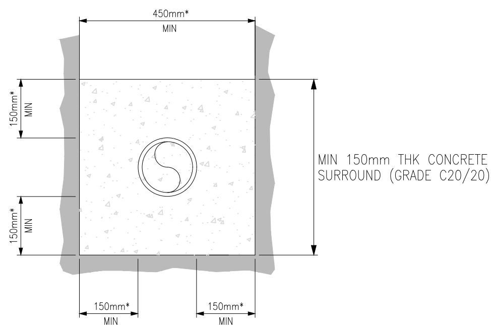
CONCRETE SURROUND (GRADE C20/20) * 100mmTHK FOR FOUL RIGID PIPES 150mmø OR LESS
