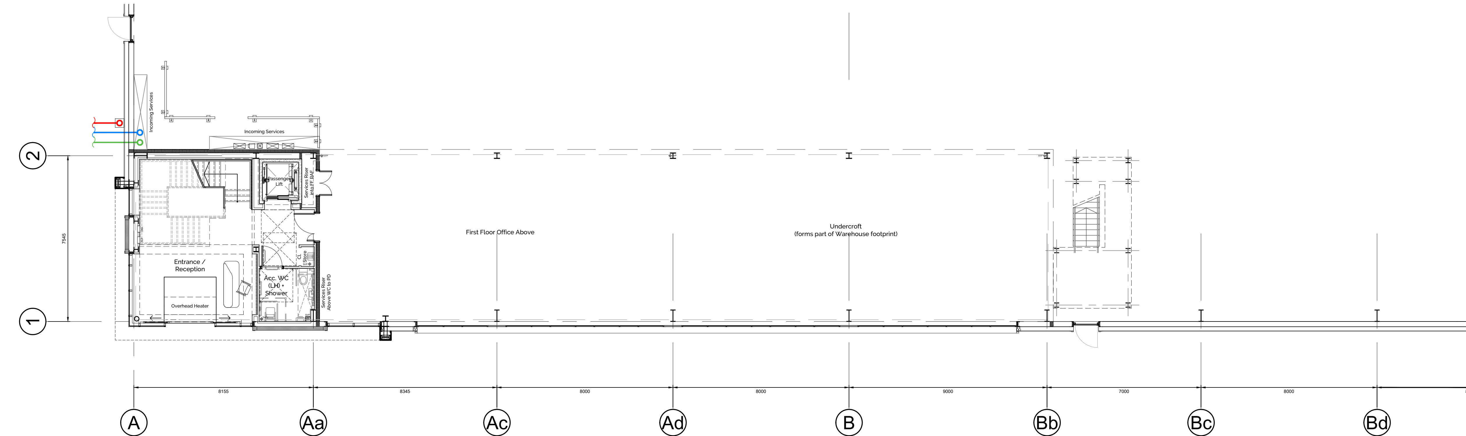
Main Office First Floor Layout +4.000m
