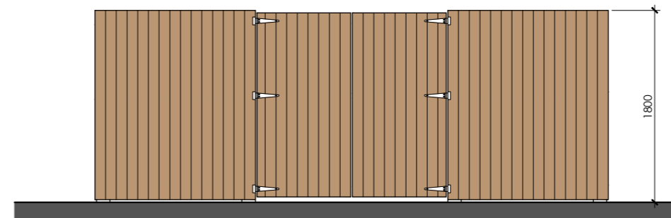
Apartments Bin Store Front Elevation Plots 67-78,79-90,91-102
