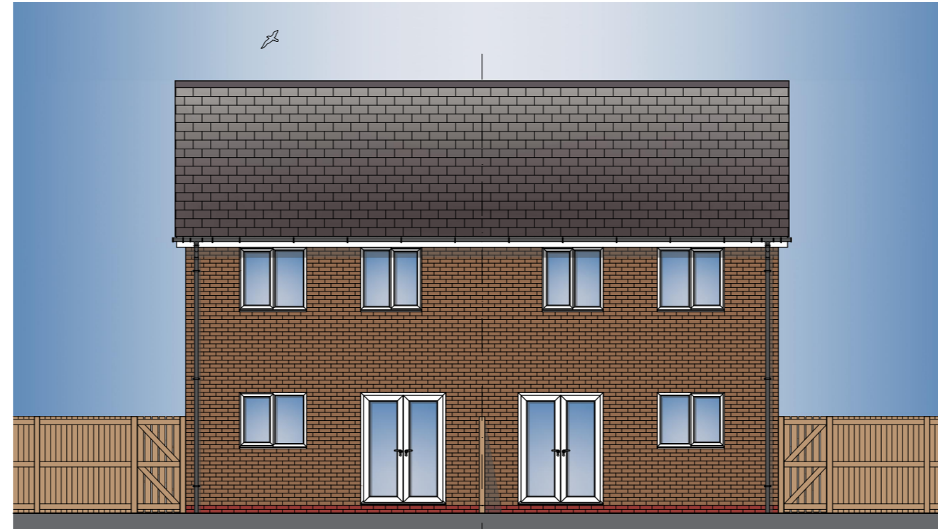
TYPE F 3B4P 86 (OPP) REAR ELEVATION - Semi-Detached
