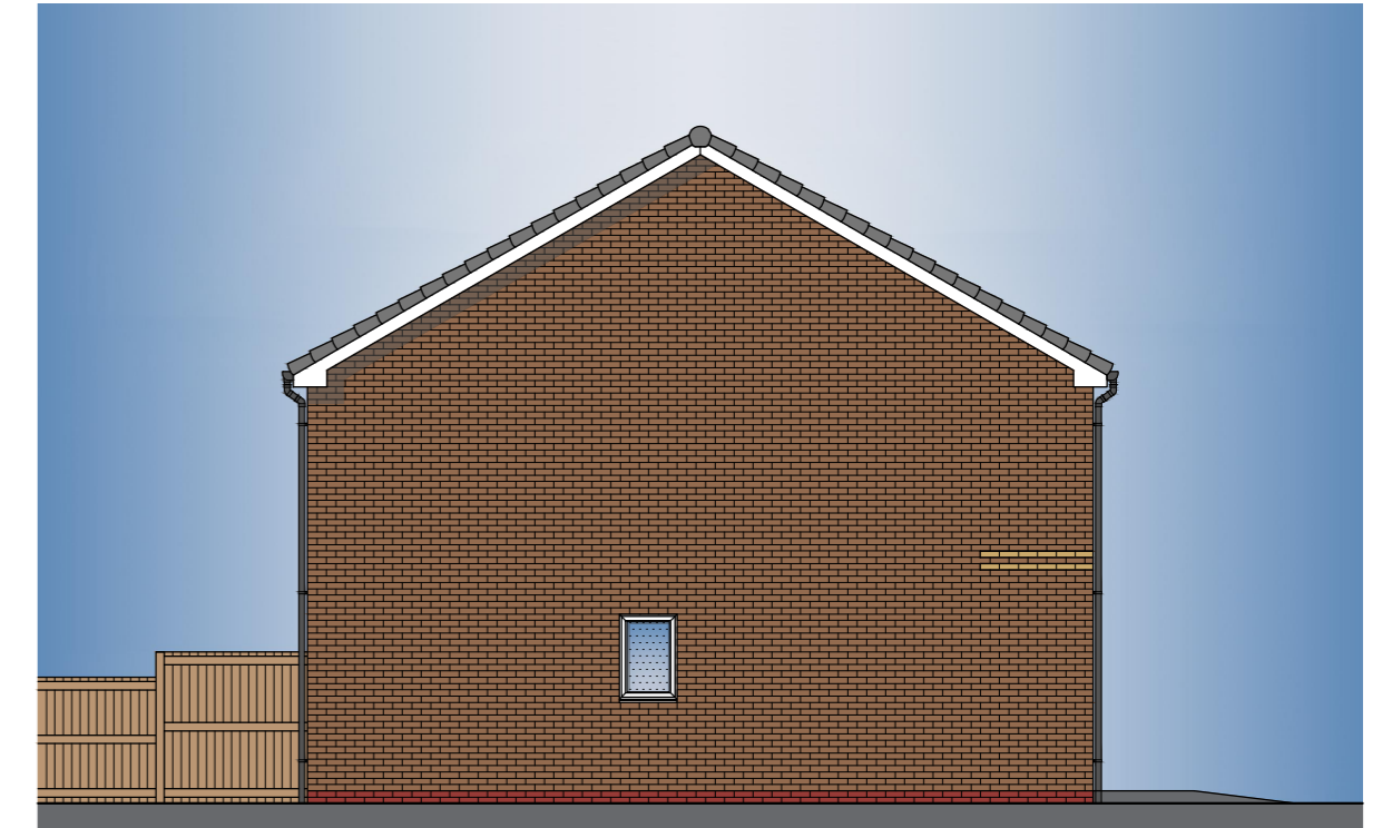
TYPE F 3B4P 86 (AS) SIDE ELEVATION - Semi-Detached
