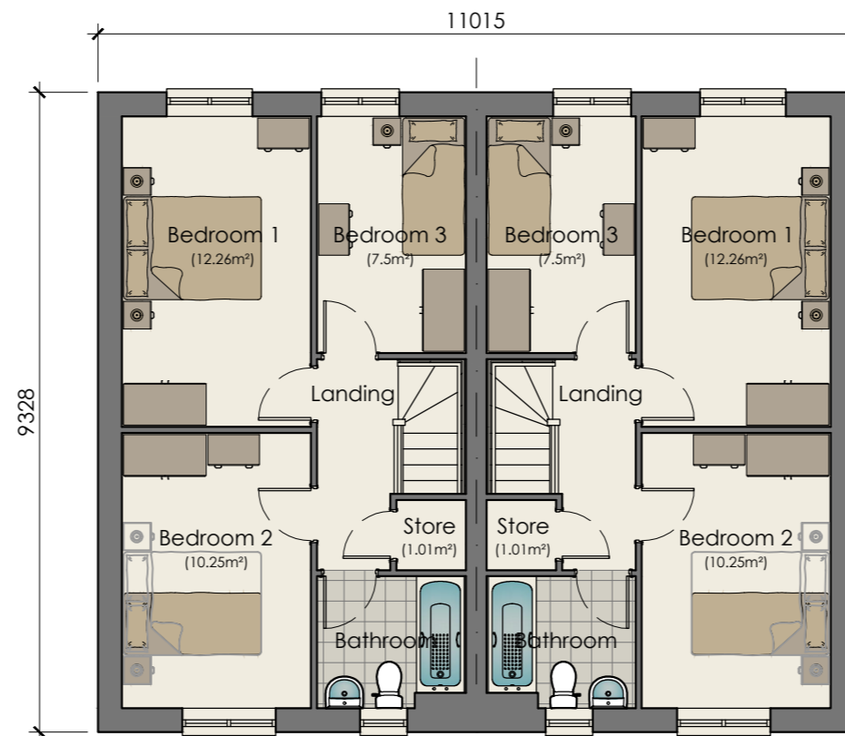
TYPE F 3B4P 86 (AS) FIRST FLOOR PLAN - Semi-Detached
