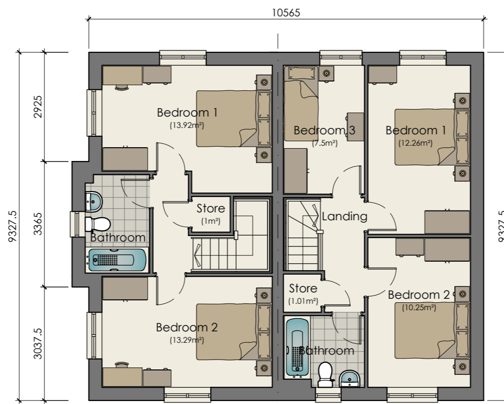
TYPE F 3B4P 86 (OPP) FIRST FLOOR PLAN - Semi-Detached
