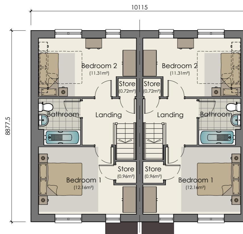
TYPE C 2B3P 74 (AS) FIRST FLOOR PLAN - Semi-Detached
