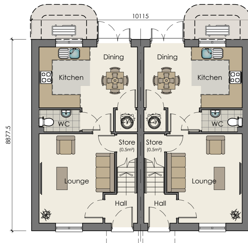
TYPE C 2B3P 74 (AS) GROUND FLOOR PLAN - Semi-Detached
