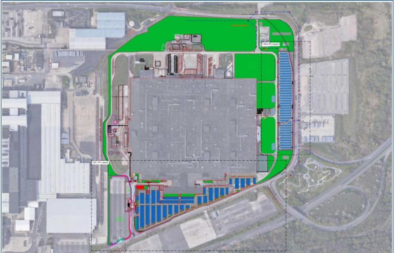
Figure 2.2 Proposed Solar Plan for the Ford Halewood Facility (extracted from Detra Solar / FM drawing OSE 1010-100)
