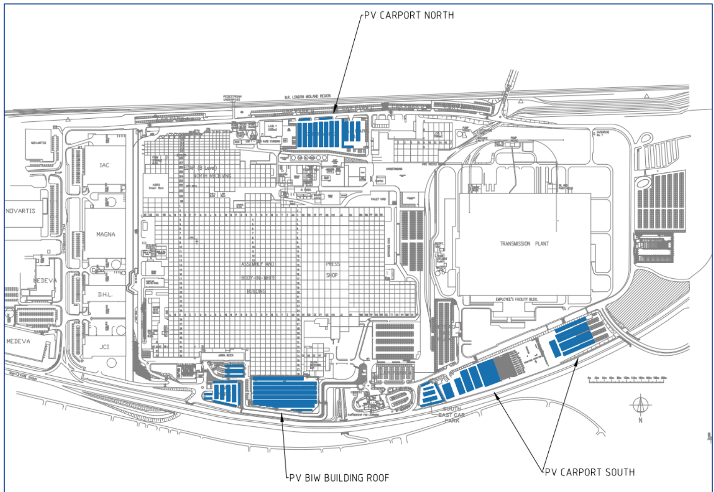
Figure 2.3: Proposed Solar Plan for the Jaguar Land Rover Facility (extracted from drawing no. LO-MEP-0020)
