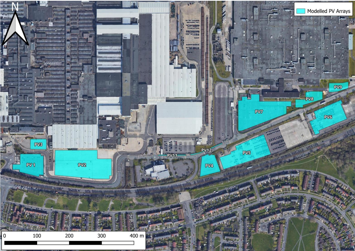
Figure 2.4: Modelled PV Arrays 1-9 and 11-12
