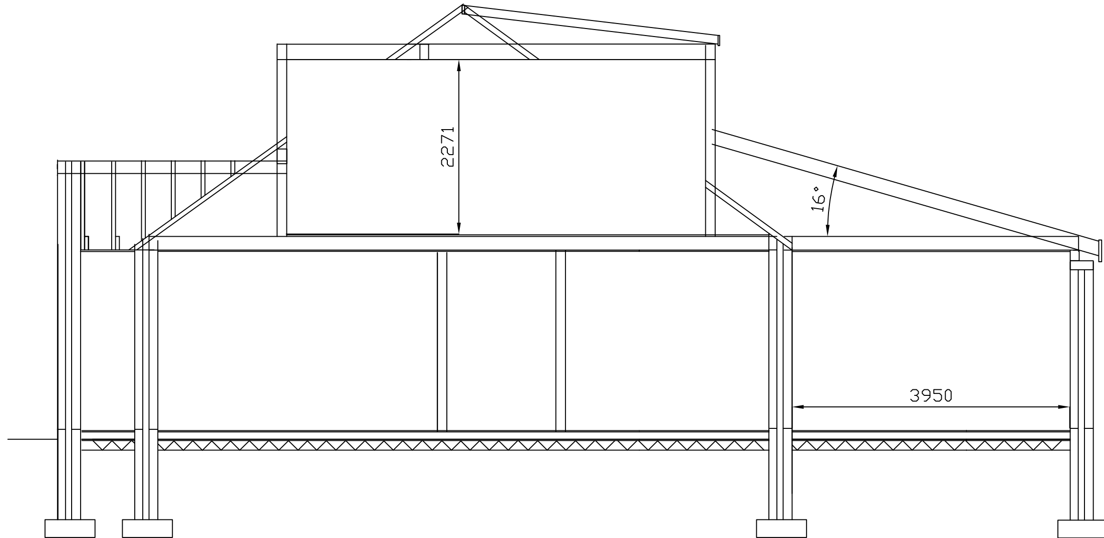
SECTION C-C
