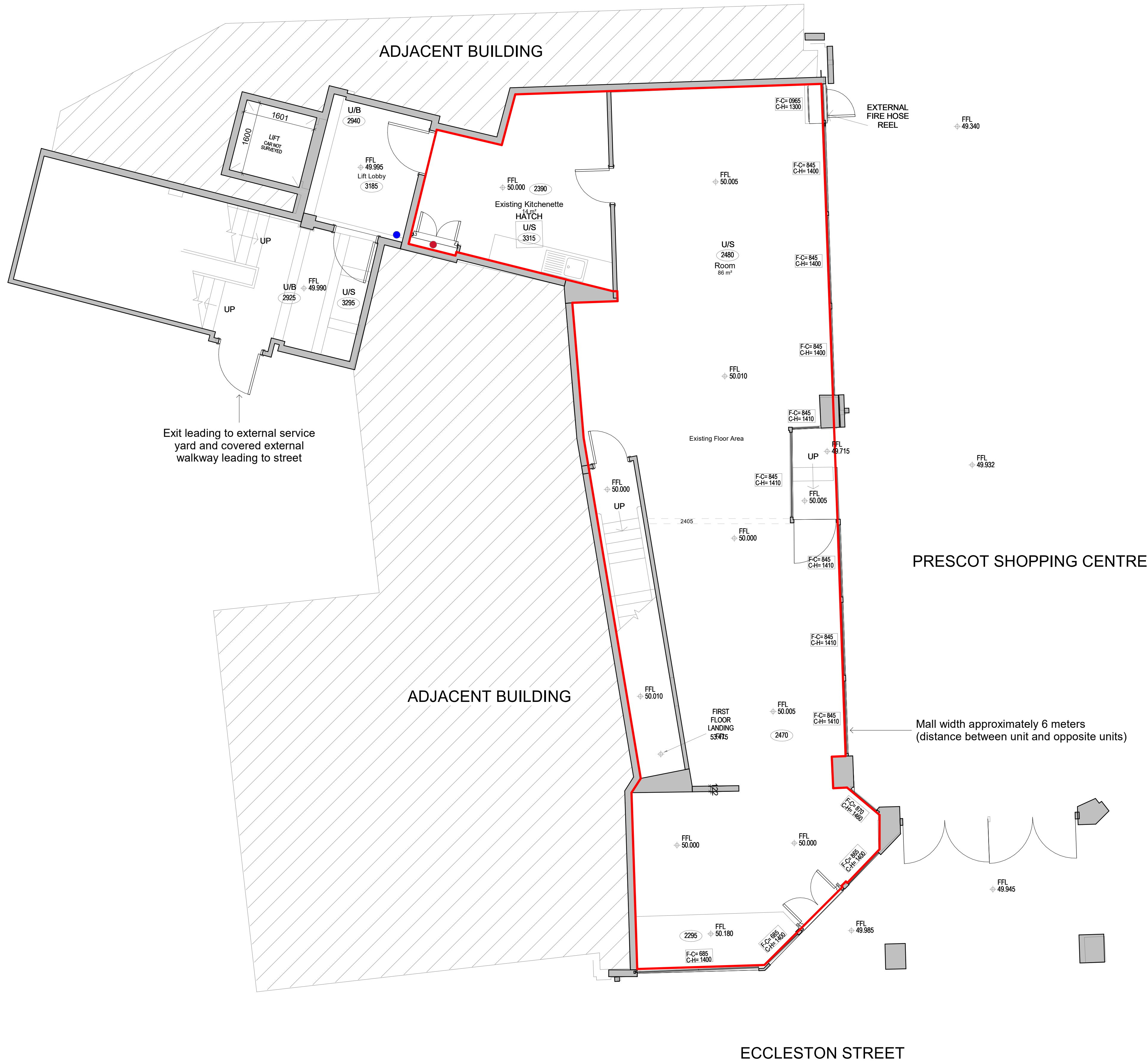
Existing Layout - Planning 1 : 50
