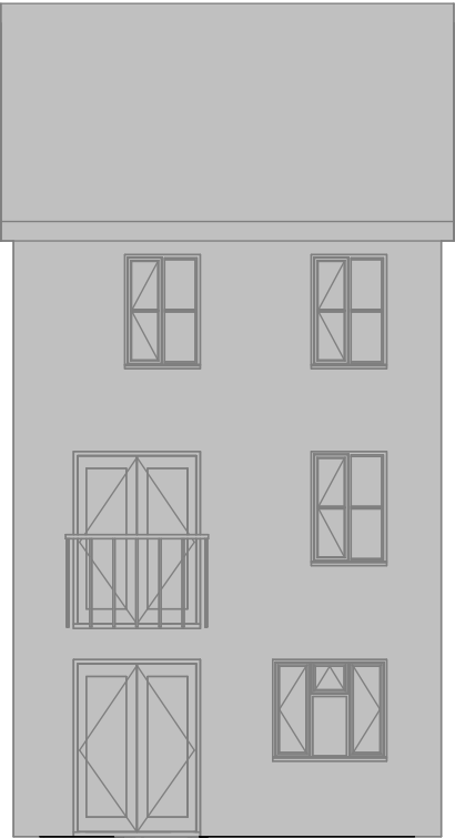
Rear Elevation 1 : 100
