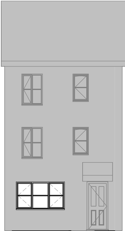
Front Elevation 1 : 100
