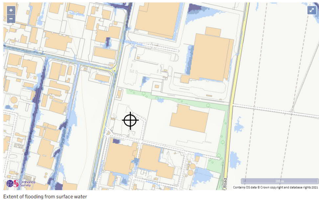
Figure 6: EA Surface Water Flood Risk Map
