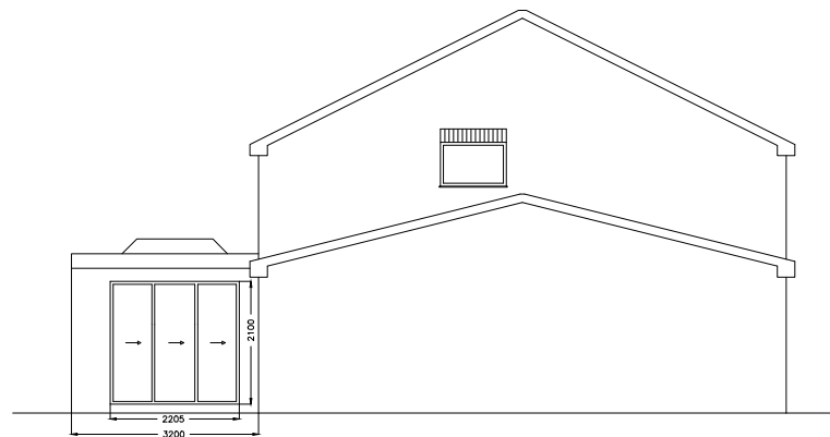
Proposed Left H/S Elevation
