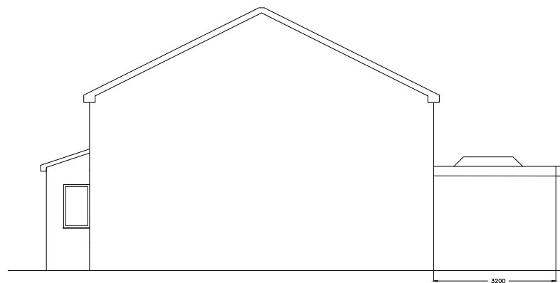
Proposed Right H/S Elevation
