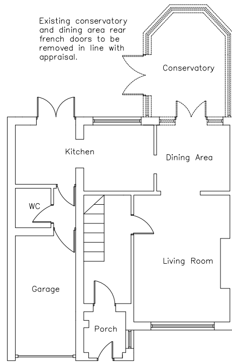
Demolition Ground Floor
