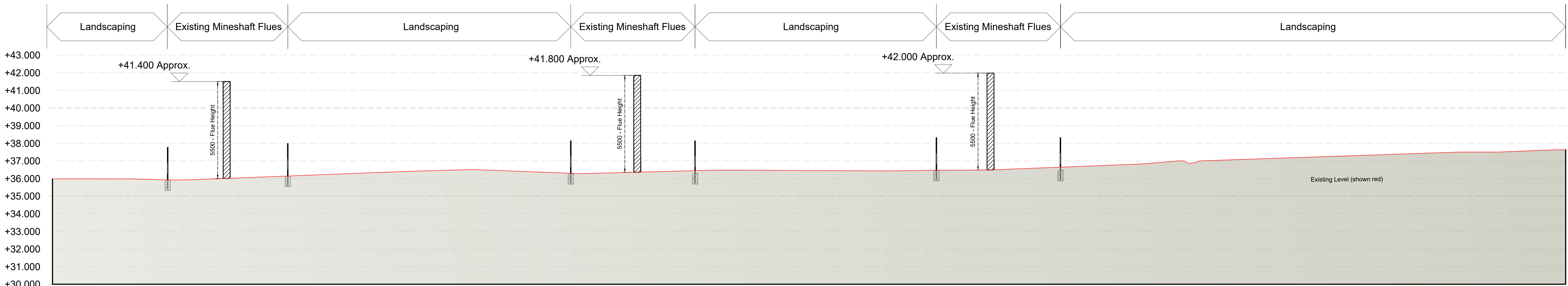
Existing Mineshaft Flues - Section A-A Scale 1:100
