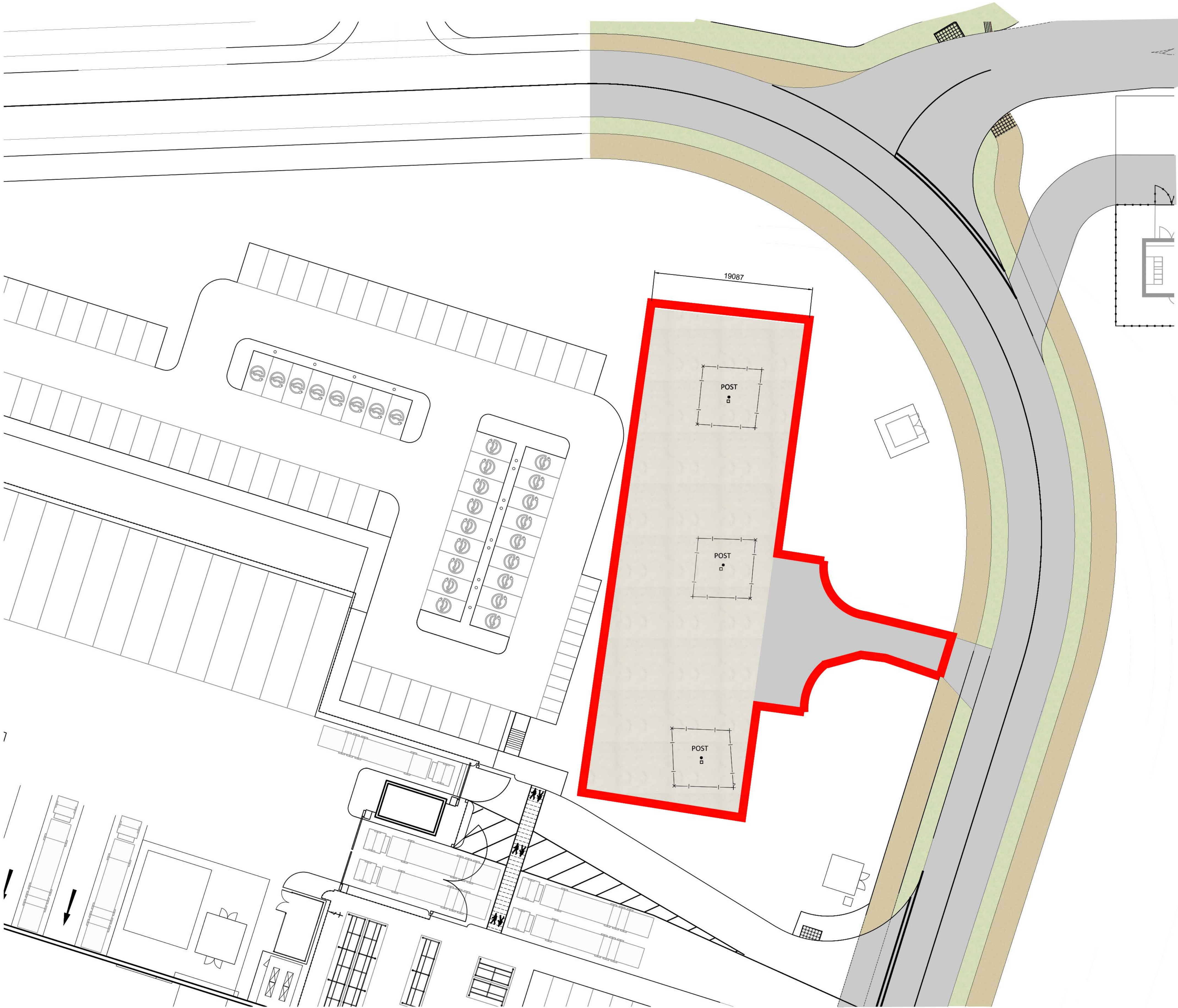
Mineshaft External Finishes Plan Scale 1:250
