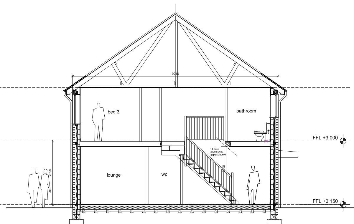
Internal section
