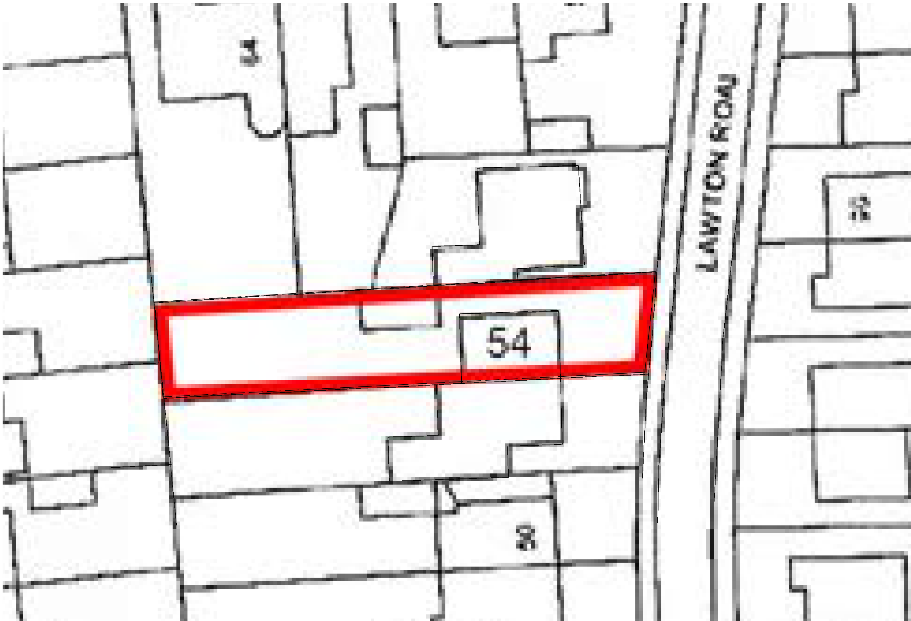
BLOCK PLAN SCALE 1:200
